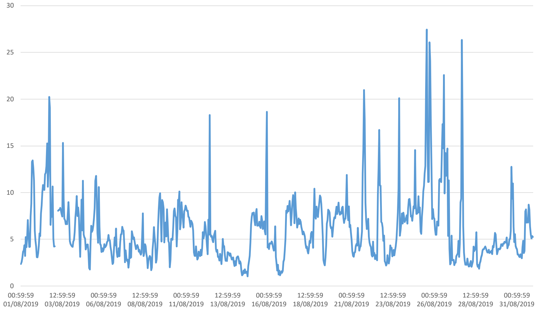
Glebe House PM10 (1-hr) emissions August ( \mu\text{g}/\text{m}^3 )
