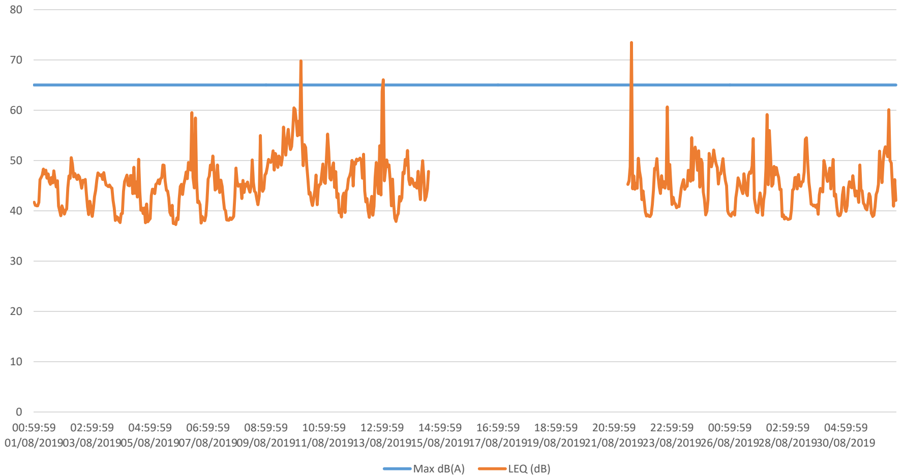
Glebe House Noise dB(A) (1hr LEQ) Aug 2019
