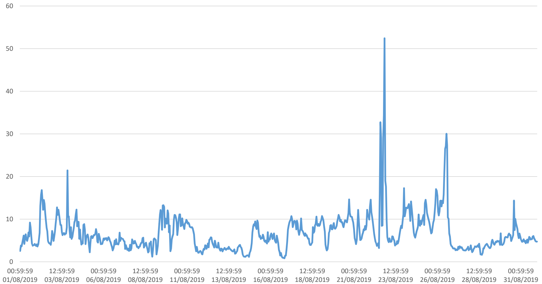
Doggetts PM10 (1-hr) emissions for August ( \mu\text{g}/\text{m}^3 )
