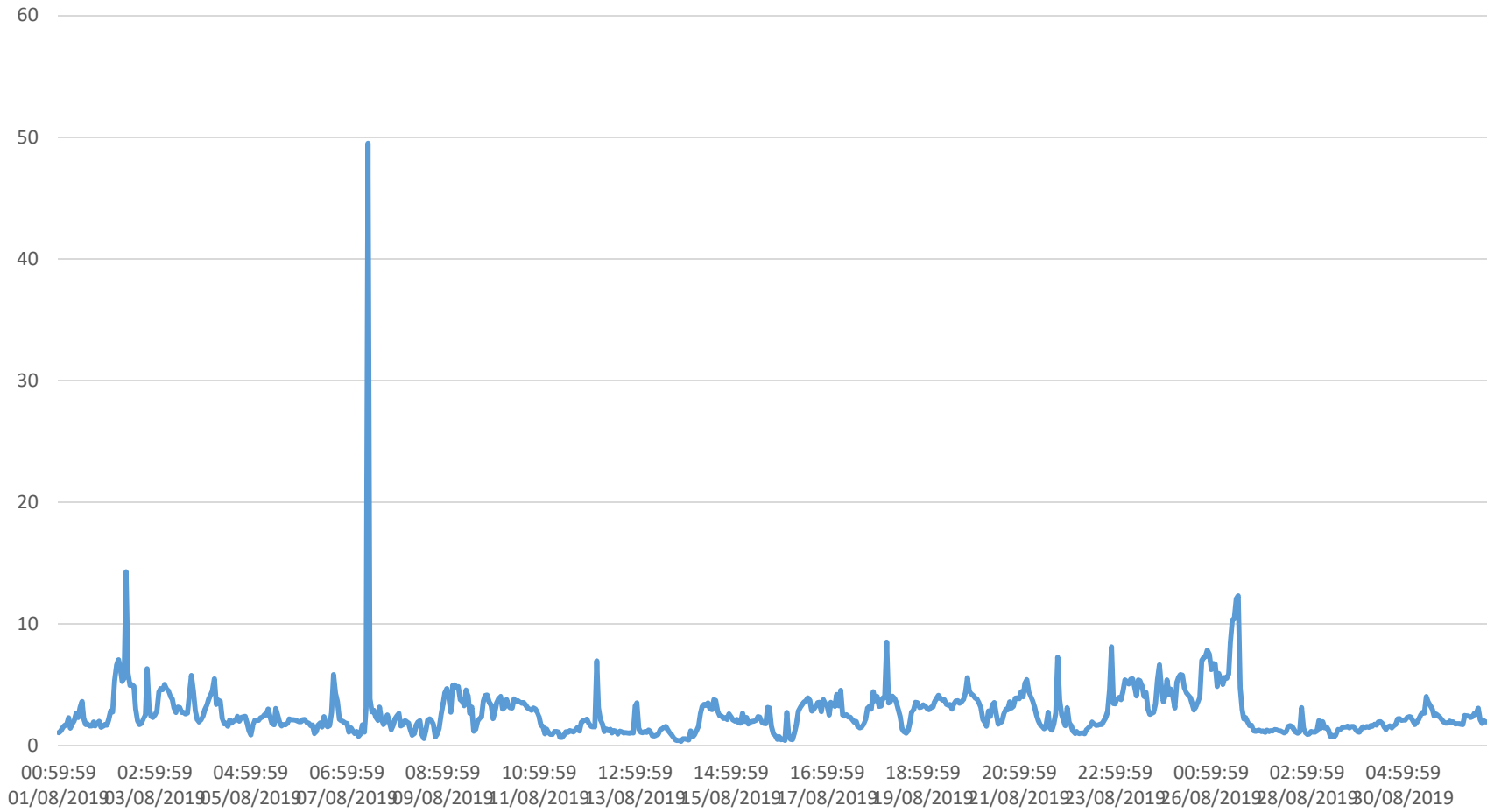
Yellow Door PM10 (1-hr) emissions for August ( \mu\text{g}/\text{m}^3 )
